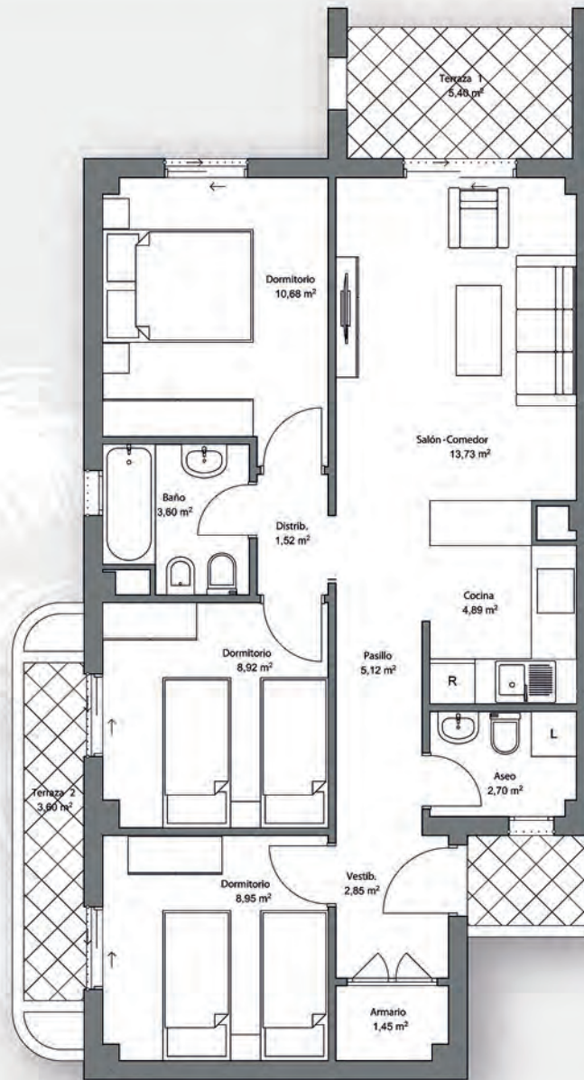
Apartment type RA2 - 3 Bedroom
